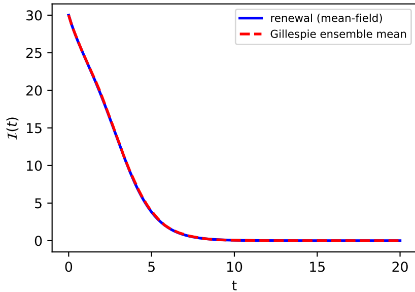
Infected cells (mu_pos)
